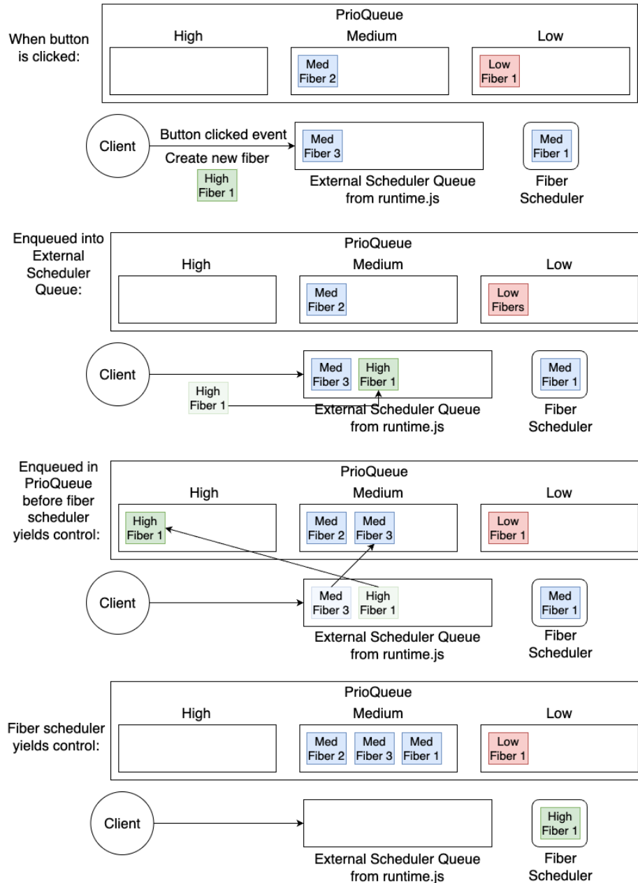
Figure 4.1: How external scheduler queue interacts with PrioQueue
