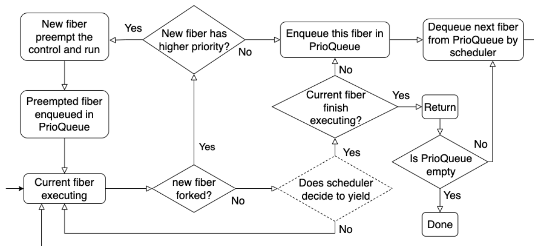
Figure 5.1: Flowchart of how the fiber scheduler operates
